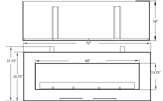
Top view & right side view of SS60 STVT61
