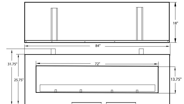
Top view & right side view of SS72 STVT73
