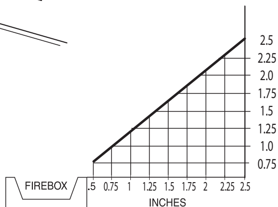
Figure 6 - Side Clearance Chart
